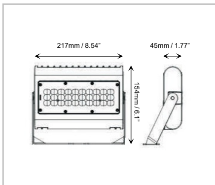
50W - U BRACKET
